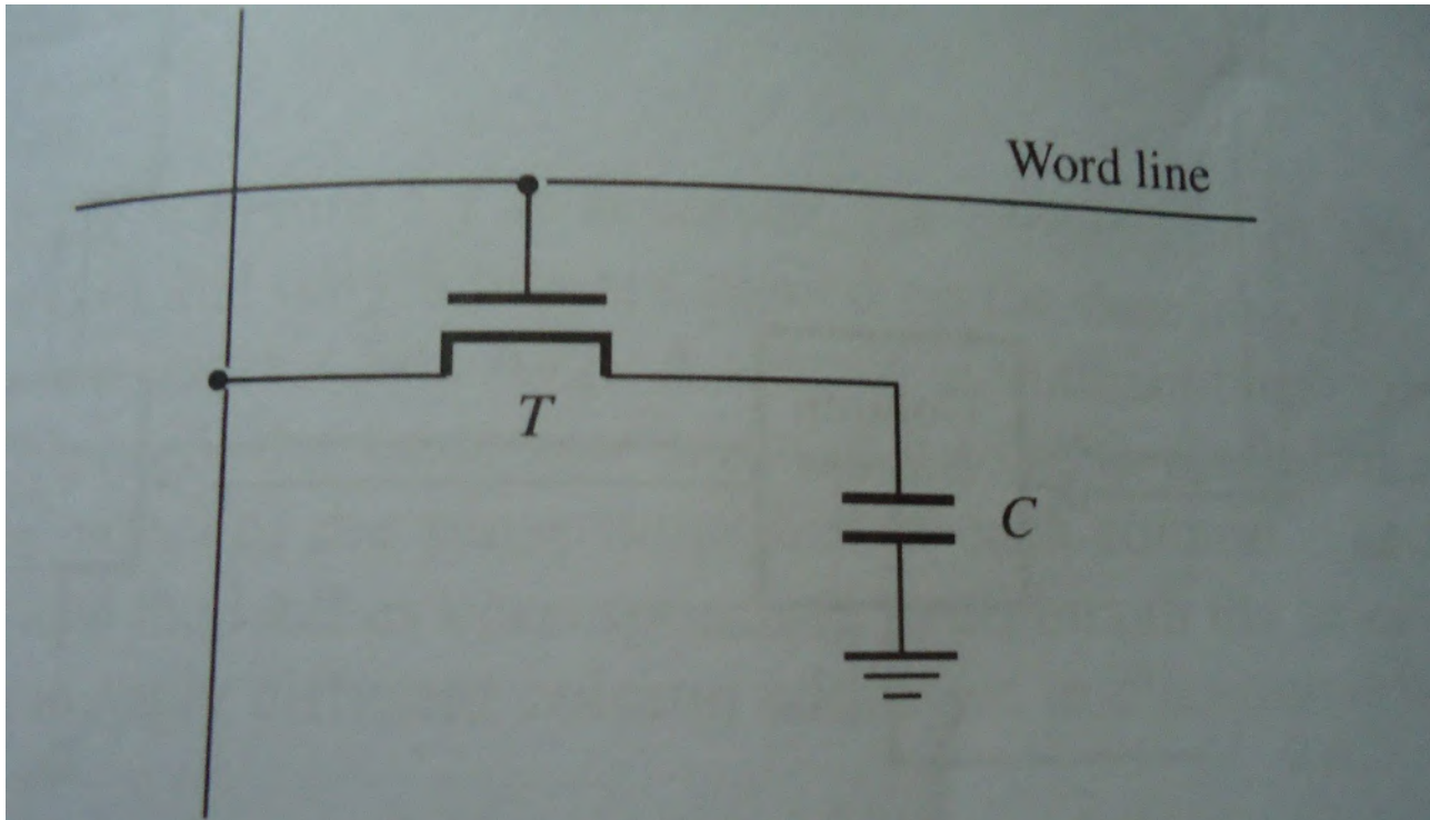
Figure 5.6 A single-transistor dynamic memory cell.
