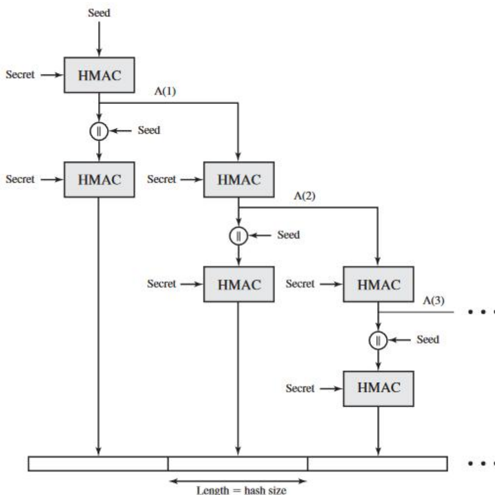
Figure 16.7 TLS Function P\_hash(\text{secret}, \text{seed})
