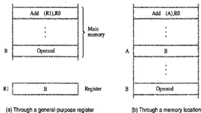
Figure 2.11 Indirect addressing.
