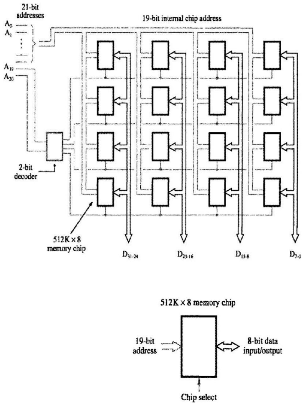
Figure 5.10 Organization of a 2\text{M} \times 32 memory module using 512\text{K} \times 8 static memory chips.
