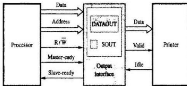
Figure 4.31 Printer to processor connection.
