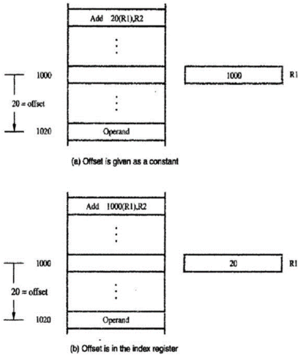
Figure 2.13 Indexed addressing.
