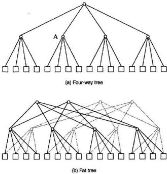
Figure 12.9 Tree-based networks.
