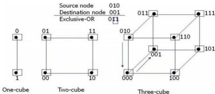
Fig: Hypercube structures for n=1,2,3
