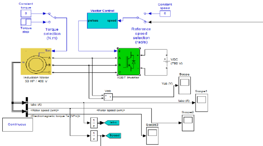
Fig 3 Vector control of induction motor
