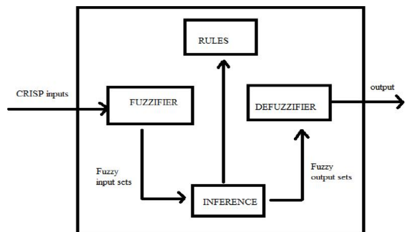
Fig 2 General block diagram of fuzzy logic controller
