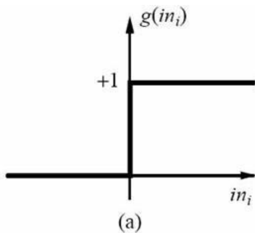
step function
